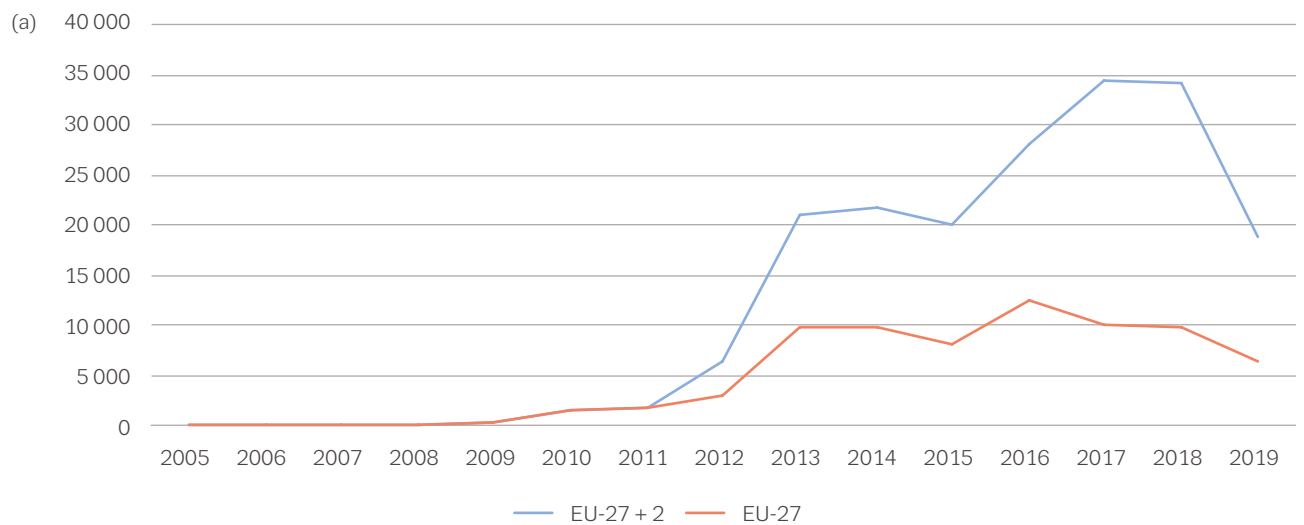
FIGURE 2 Seizures of synthetic cannabinoids reported to the EU Early Warning System: trends in (a) the number of seizures of synthetic cannabinoids and (b) the quantity seized, in weight (kg), 2005–2019 (all forms including powders and herbal smoking mixtures – EU-27 and EU-27 + 2)
