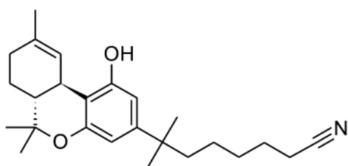
FIGURE 4 Chemical structure of O -774
