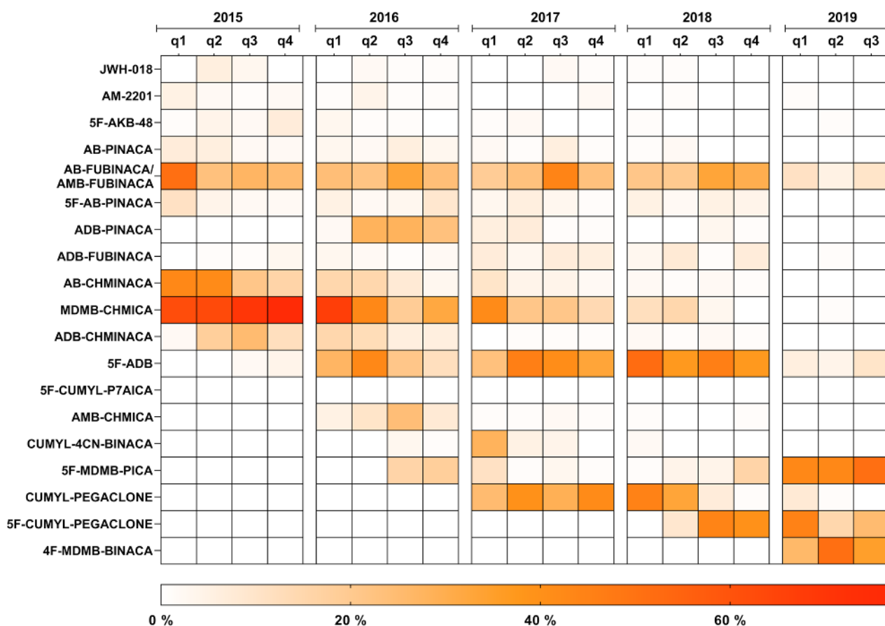
FIGURE 3 Heat map presenting the relative positivity rate of 20 selected synthetic cannabinoids in urine samples analysed in the Institute of Forensic Medicine Freiburg (Germany), 2015 to 2019
