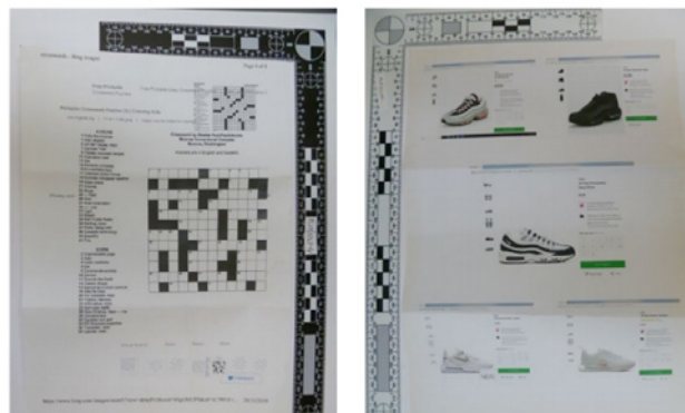
FIGURE 7 A4-sized printouts, seized in a prison in Scotland, United Kingdom, during 2019, that were impregnated with MDMB-4en-PINACA and 5F-MDMB-PICA
