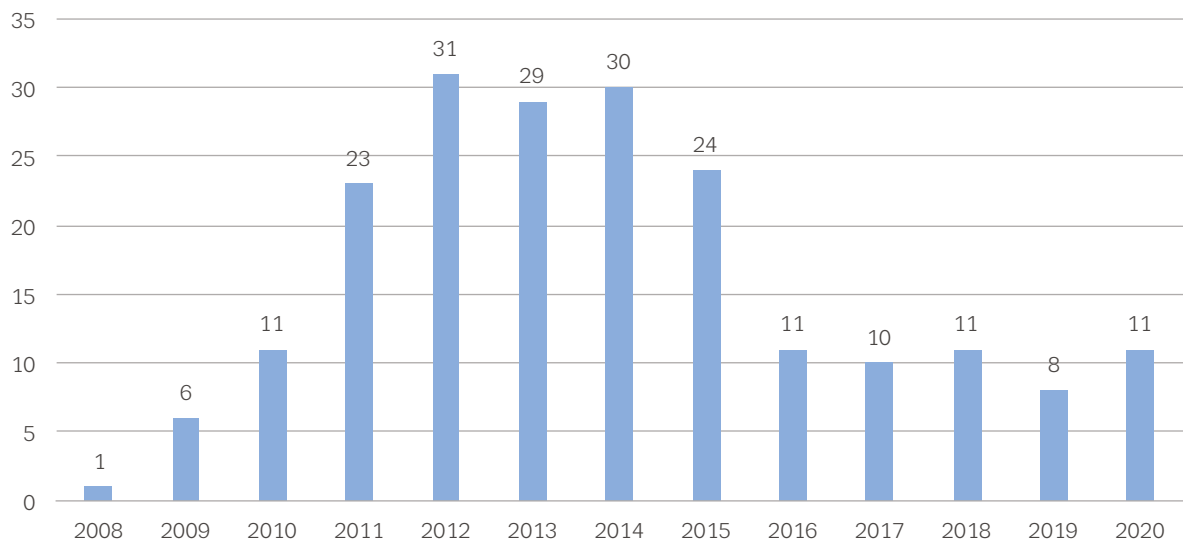
FIGURE 1 Number of synthetic cannabinoids formally notified to the EU Early Warning System for the first time, 2008–2020
