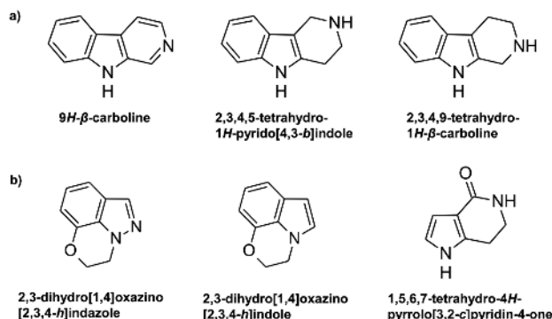
FIGURE 5 Potential core structures of synthetic cannabinoids that might be used for the production of new psychoactive substances, as proposed by (a) Diaz et al. (2017) and (b) Leftheris et al. (2003)
