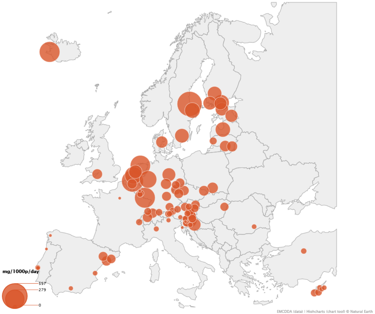
Figure 8. Relative geographical distribution of amphetamine residues as detected in European cities, 2023 (daily mean)
