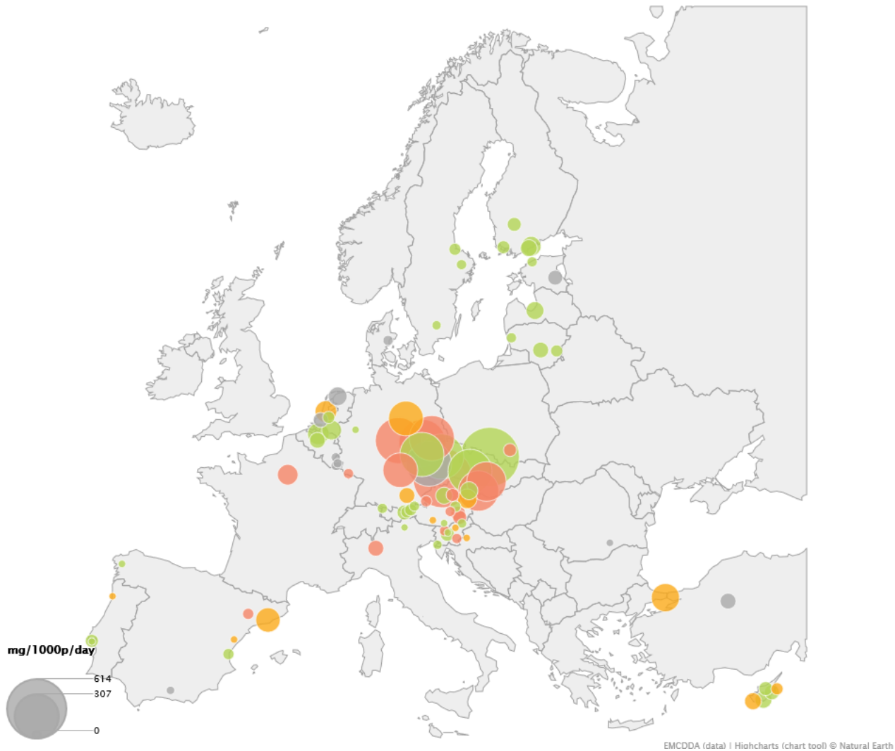
Figure 11: Changes in the mean weekly methamphetamine metabolites from wastewater analyses in selected European cities between 2022 and 2023 Red = increase | Green = decrease | Yellow = stable, with respect to previous year
