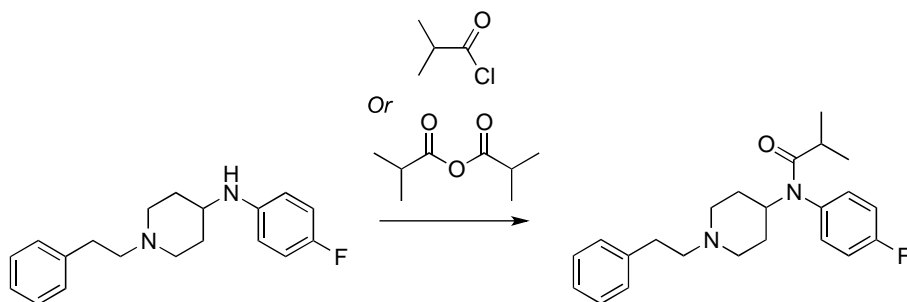
Figure 2. A possible final step of the synthesis of 4-fluoroisobutyrylfentanyl employing the acylation of the N -(4-fluorophenyl)-1-(2-phenylethyl)piperidin-4-amine intermediate using either isobutyryl chloride or isobutyric anhydride.
