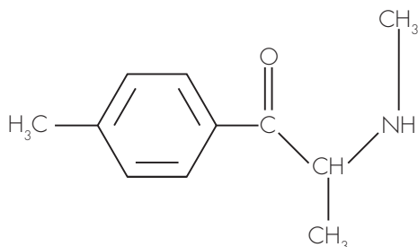
Figure 1 – Chemical structure of mephedrone
